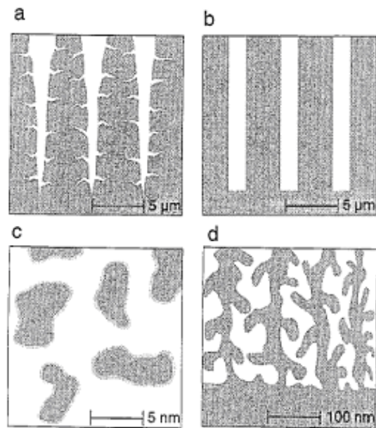
Fig-1: Effects of variations in etch parameters on pore geometry
