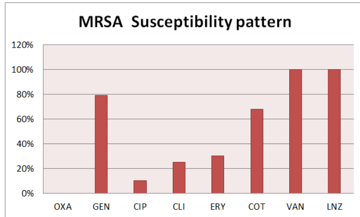
Graph-1: Graph showing MRSA antibiotic sensitivity pattern
