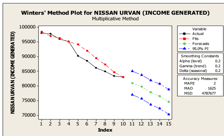
Fig-3: Winters' Method Plot for Nissan Urvan (Income Generated)
