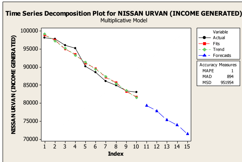
Fig-1: Time Series Decomposition Plot for Nissan Urvan (Income Generated)
