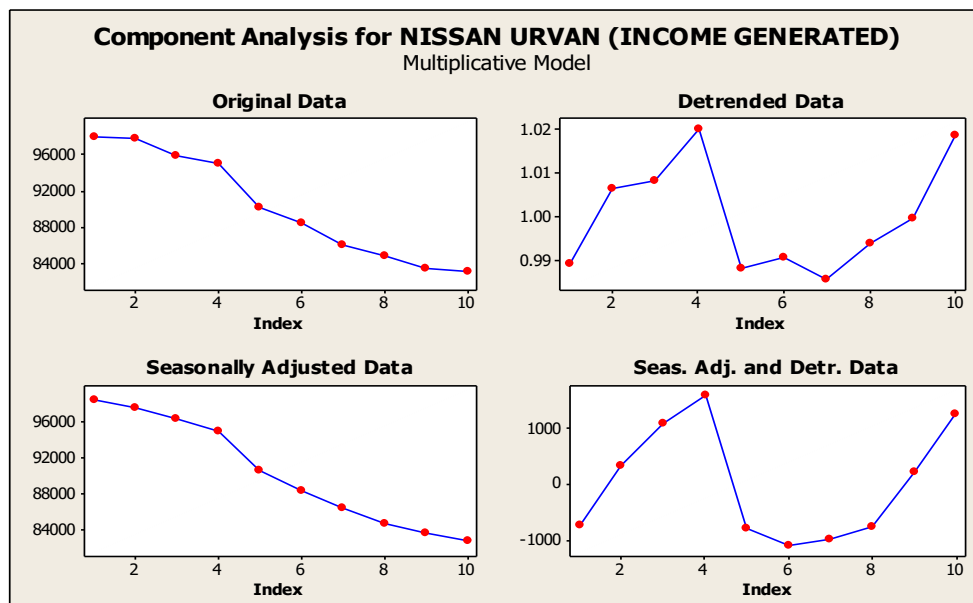
Fig-2: Decomposition - Component Analysis for Nissan Urvan (Income Generated)
