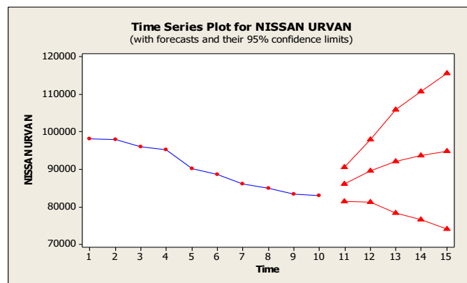
Fig-4: Time Series Plot for Nissan Urvan
