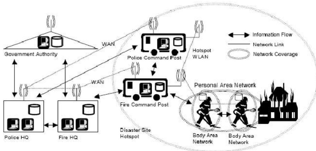
Fig-1: Communication architecture schematic
